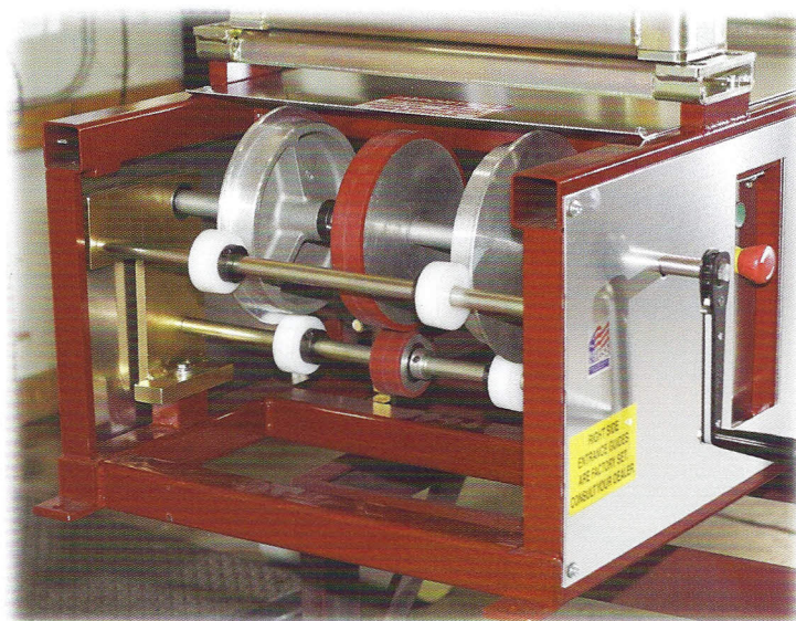
Easy feed entrance guide
